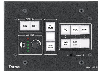
Control Box
